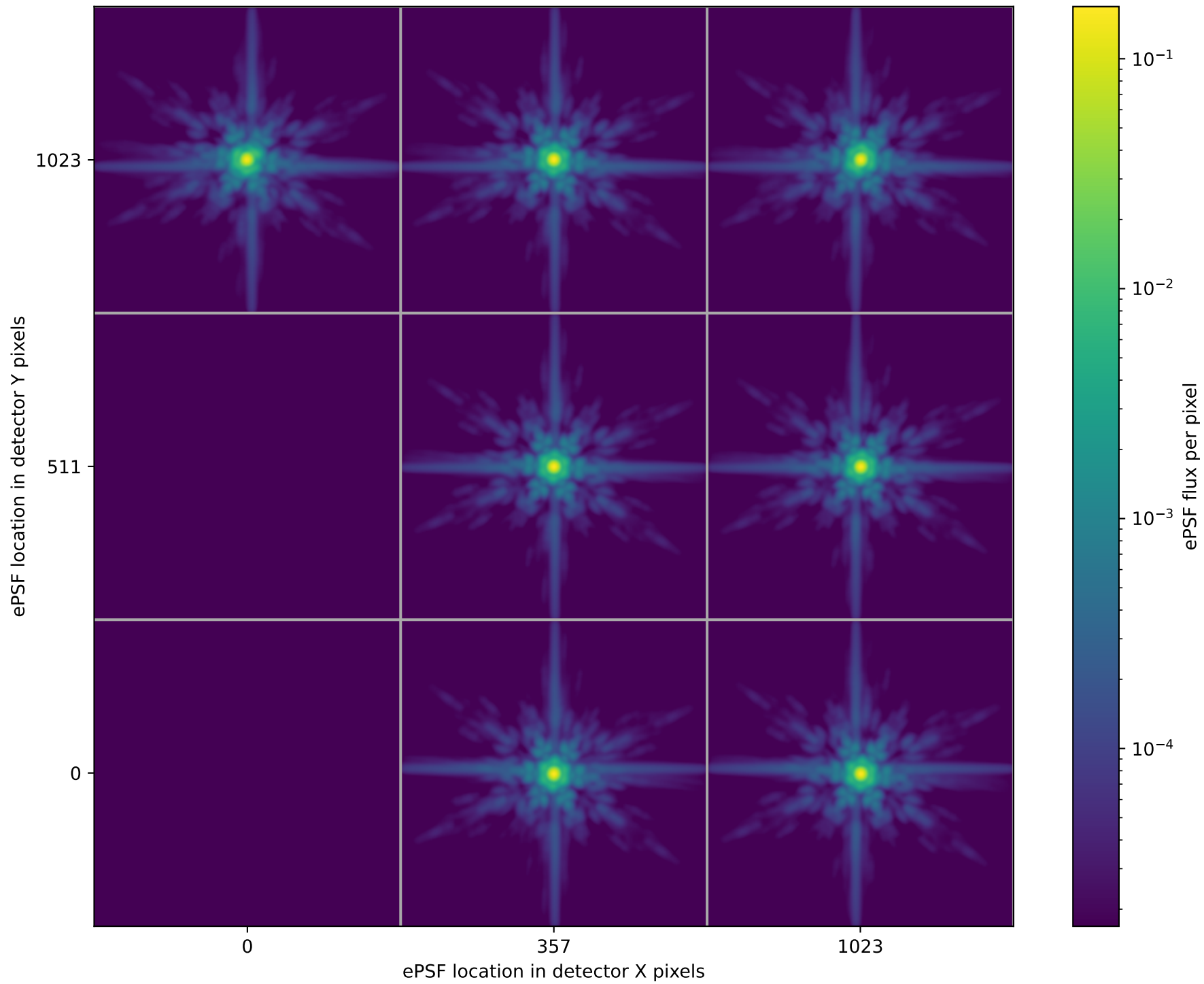
MIRI MIRIM F560W ePSFs
