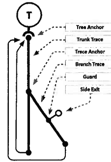
Figure 5. A tree with two traces, a trunk trace and one branch trace. The trunk trace contains a guard to which a branch trace was attached. The branch trace contains a guard that may fail and trigger a side exit. Both the trunk and the branch trace loop back to the tree anchor, which is the beginning of the trace tree.
