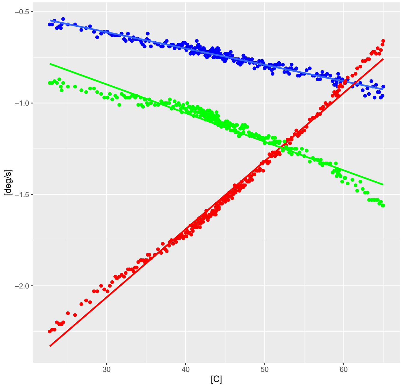
Hub RX angular velocity vs temperature
