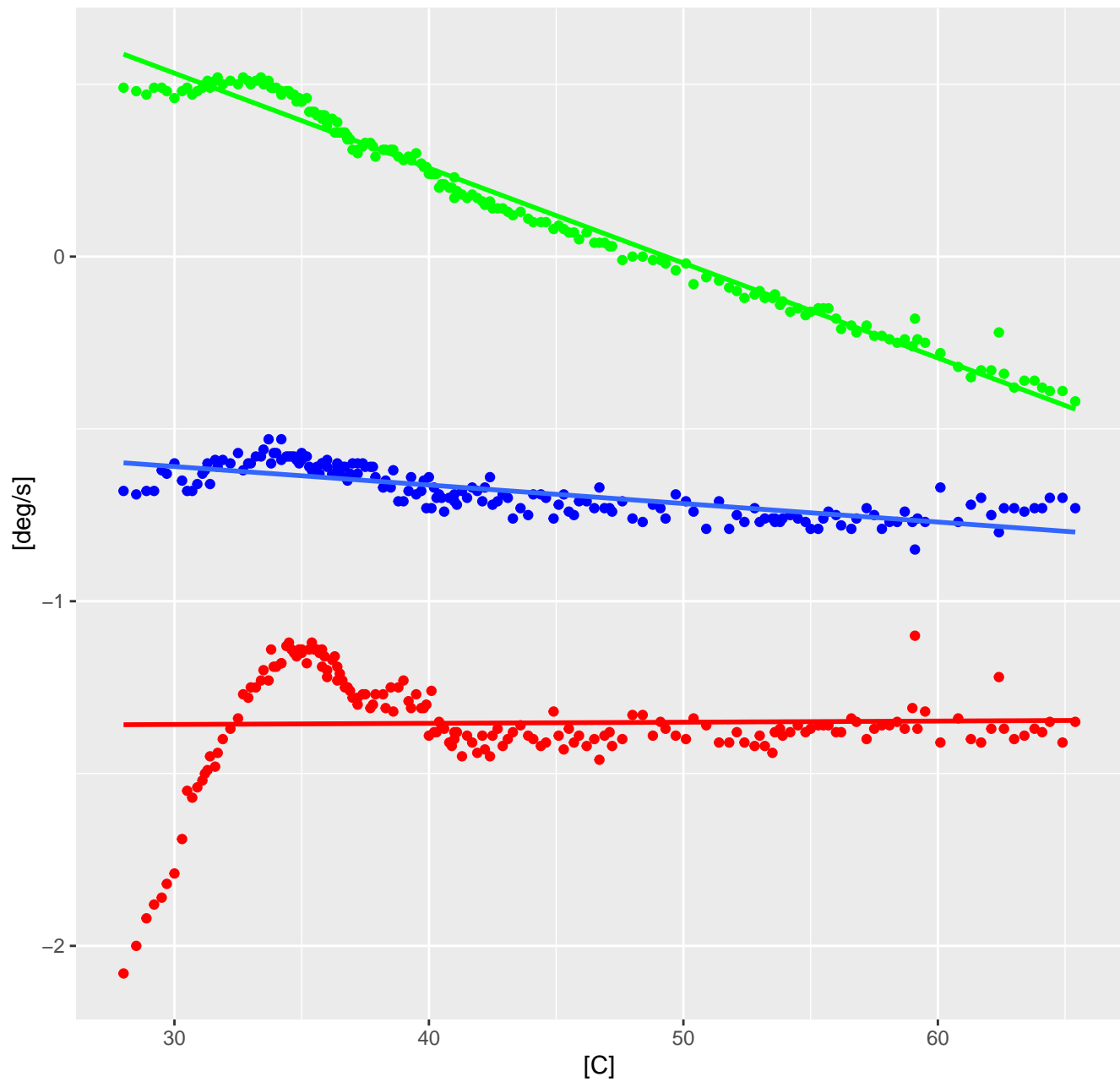
Hub RG angular velocity vs temperature
