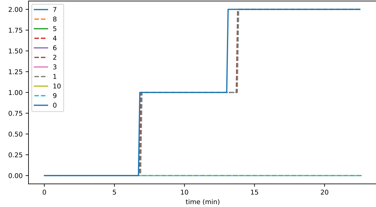
vmap_lifecycle_flushCount_accounts
