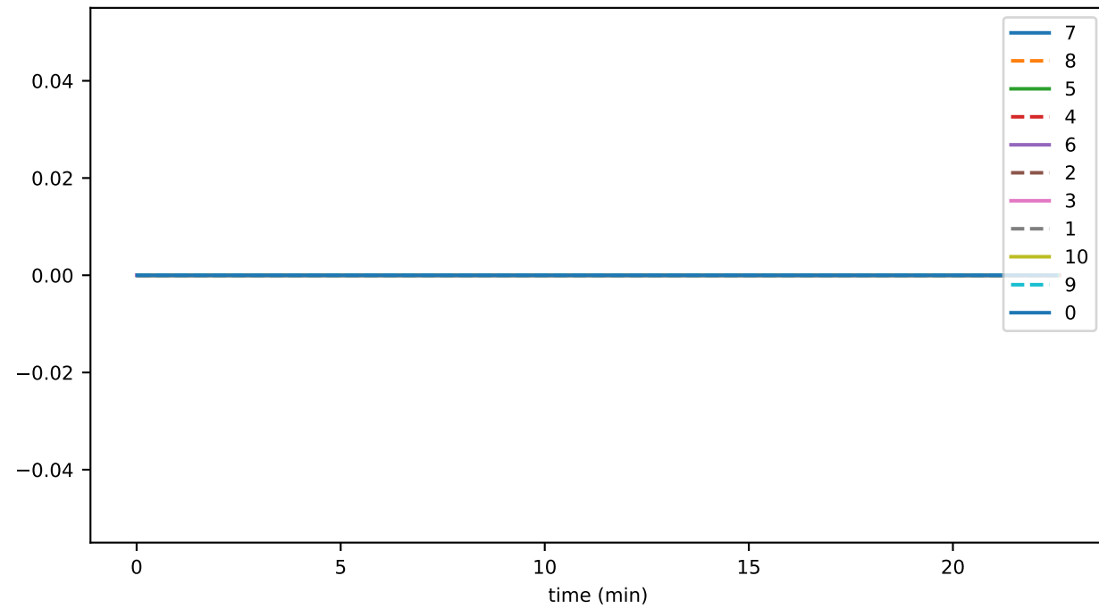
ds_files_level_3_leafKeysFileSizeByLevelMb_accounts
