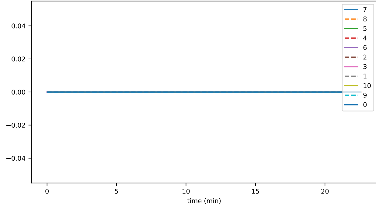
disconnects_per_sec_01
