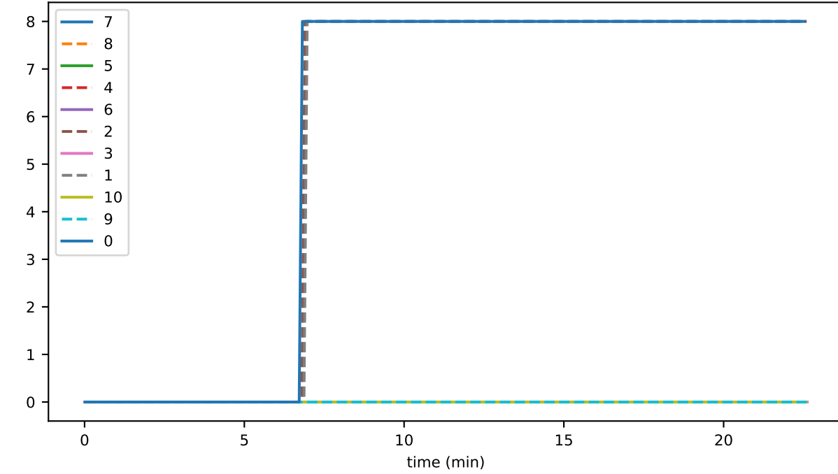
ds_offheap_objectKeyBucketsIndexMb_accounts
