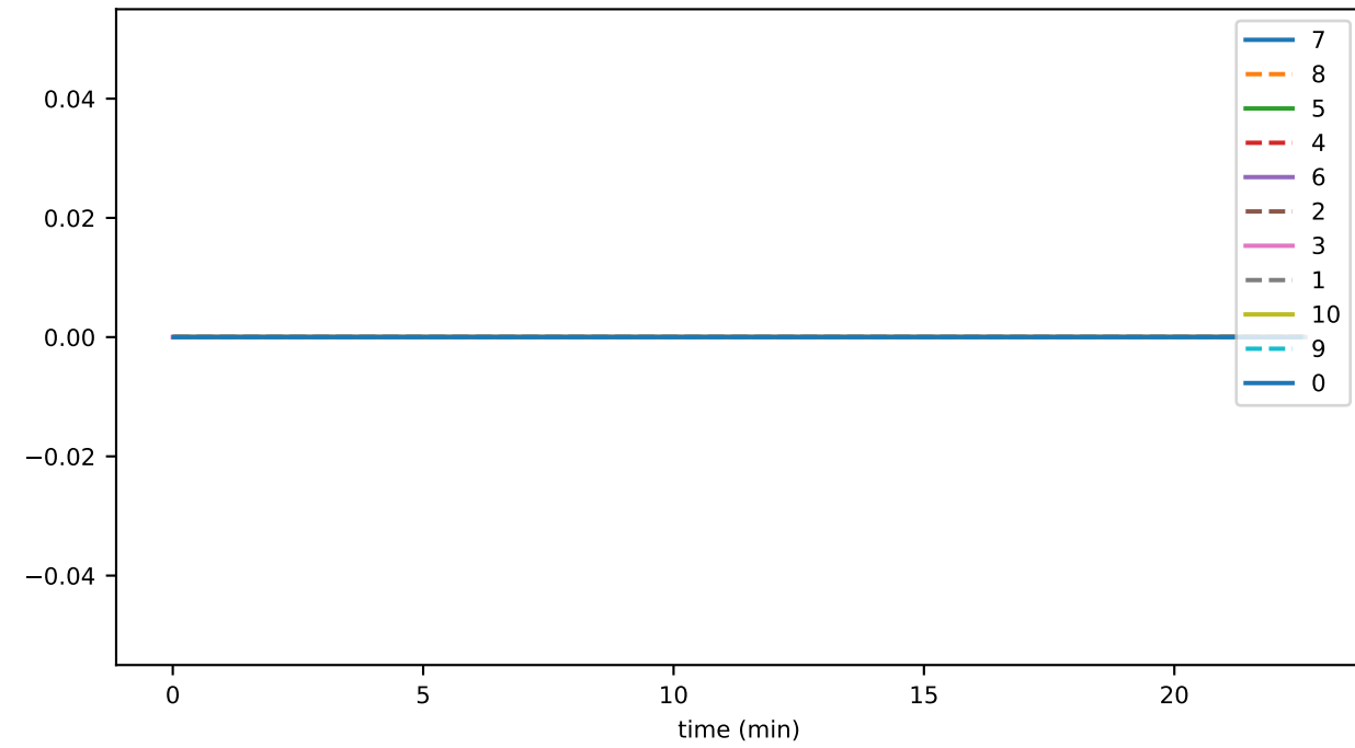
parentGenerationMismatch
