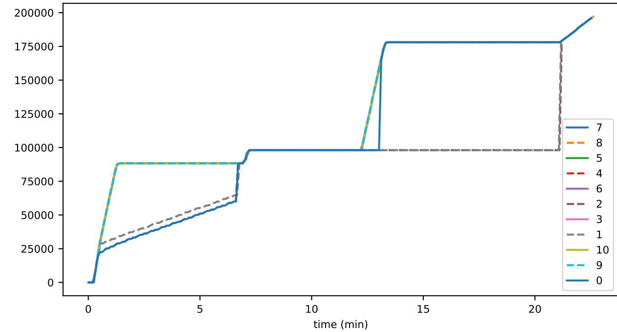
vmContractExecute
