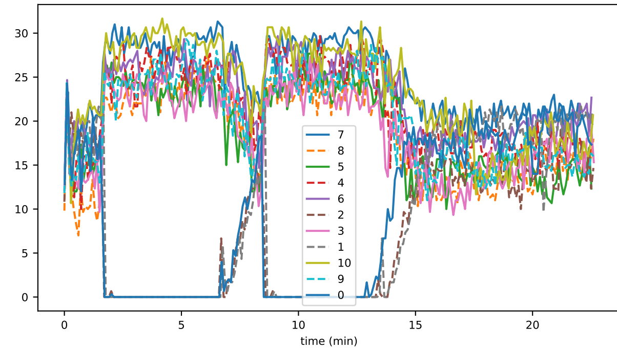
parentGenerationMismatch
