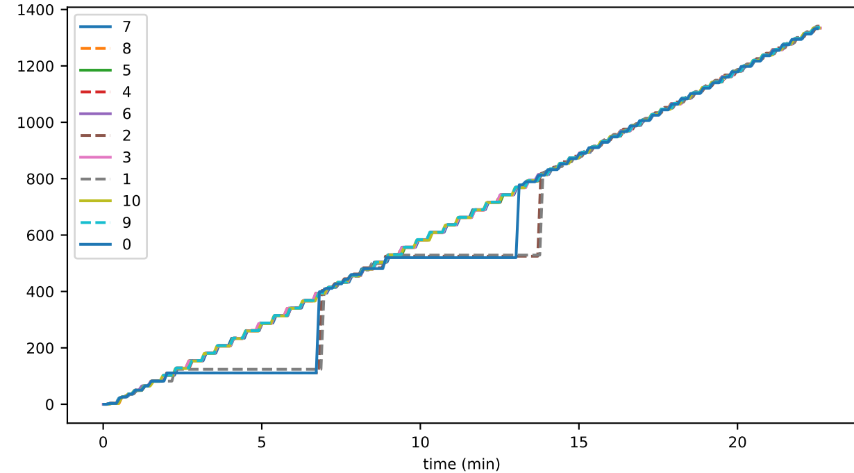
preconsensusEventFileOldestSeconds
