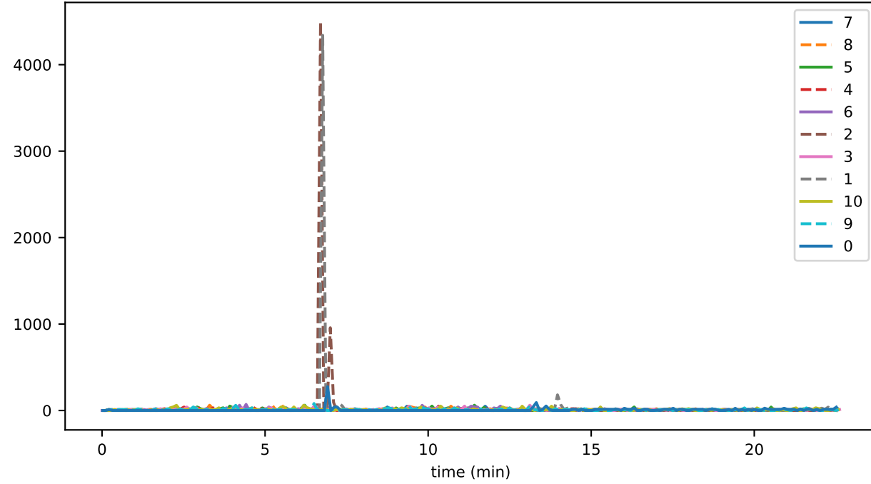
bufferedTransactions
