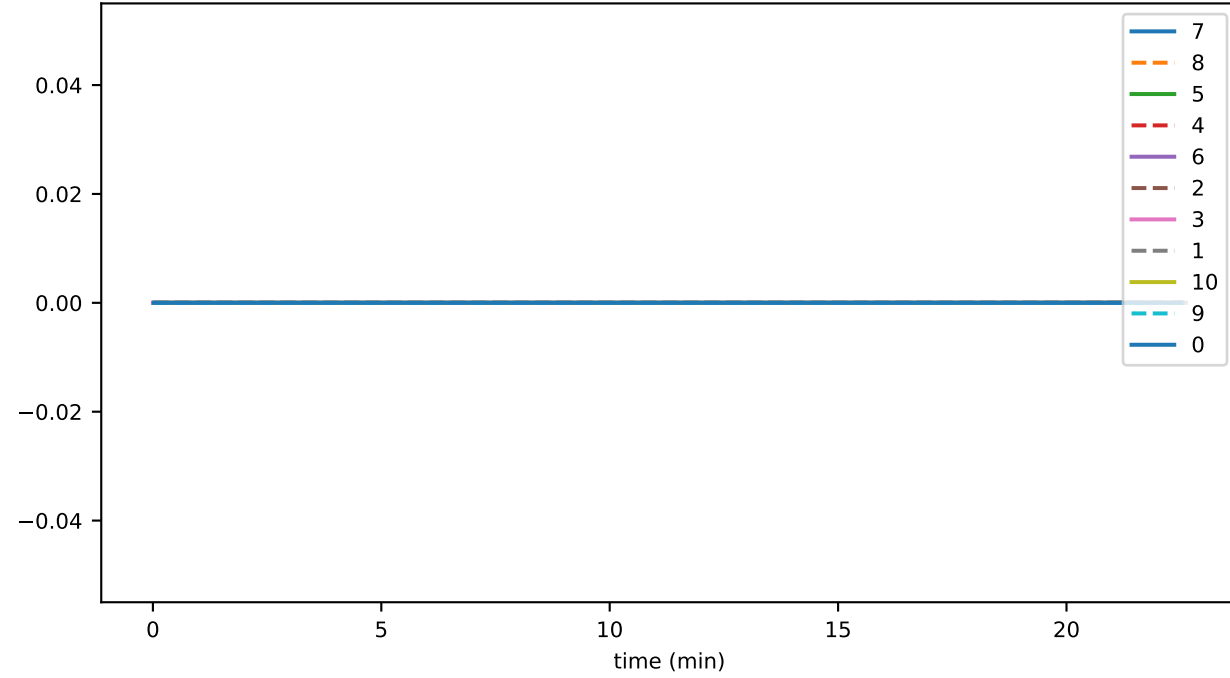
ds_files_level_0_leavesFileSizeByLevelMb_accounts
