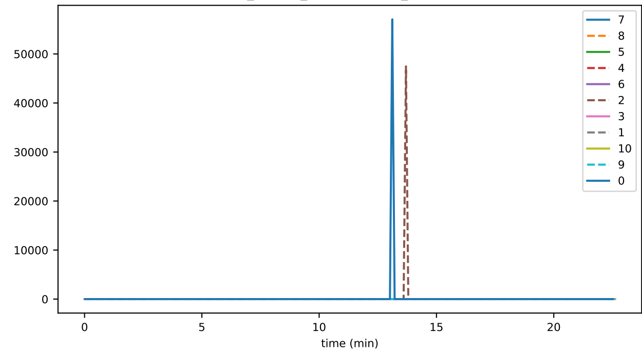
ds_flushes_leavesDeleted_accounts
