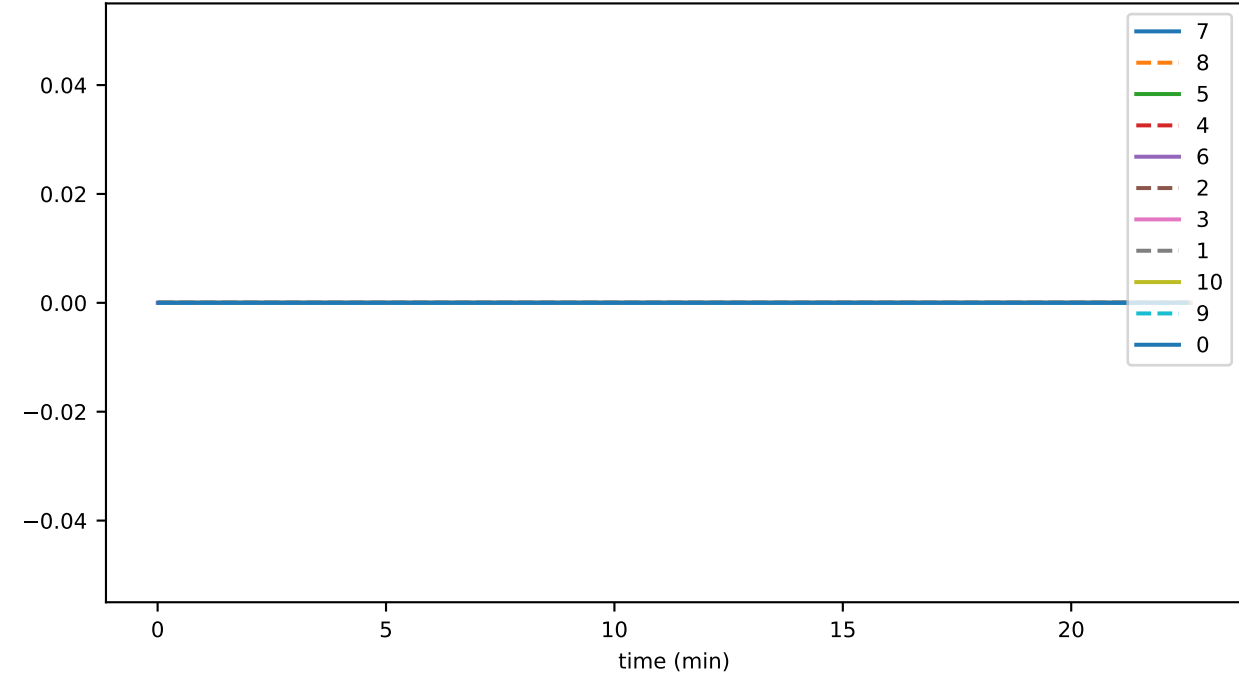
oldestBlockingSwirdStateSeconds
