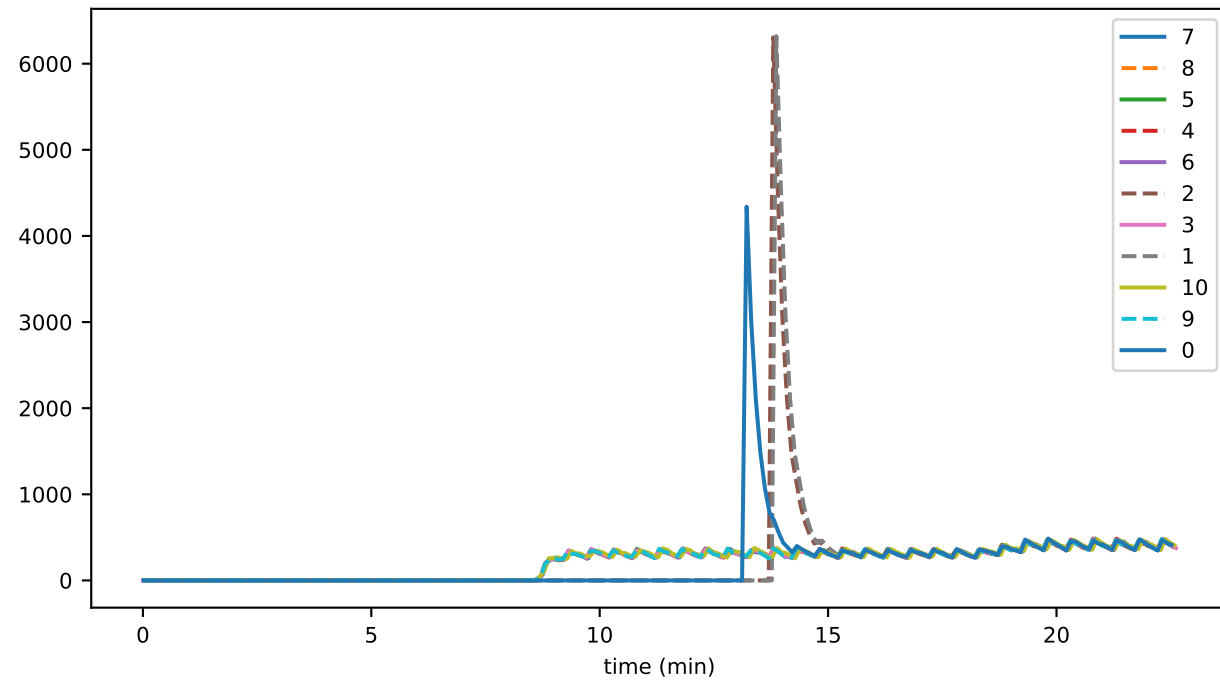
fcqHashExecMicroSec
