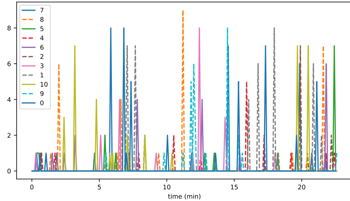
transferredTokensPerSecond
