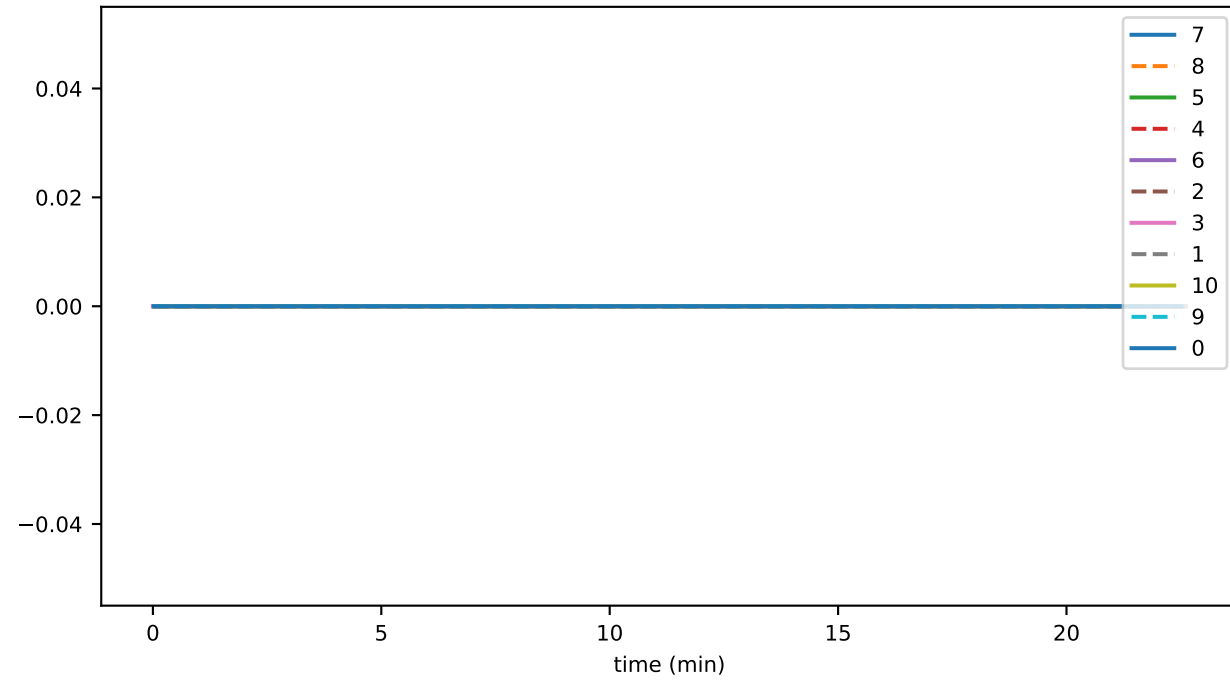
bufferedTransactions
