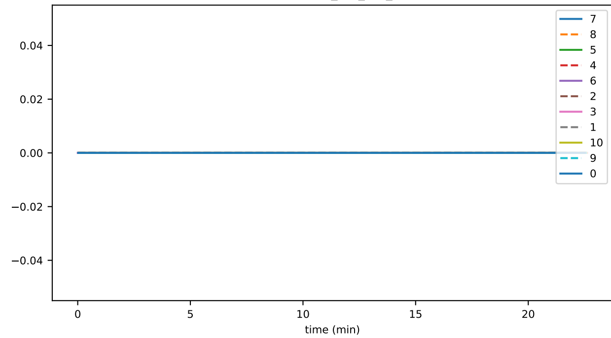
disconnects_per_sec_05
