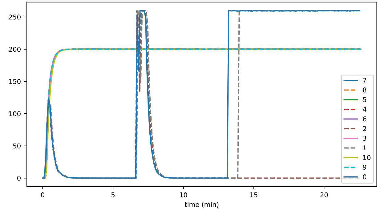
averageTimeToFullySignState
