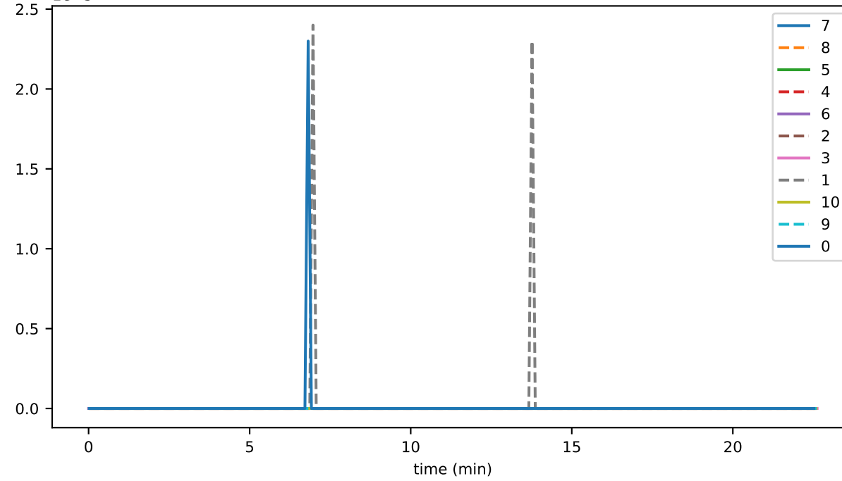
ds_flushes_hashesStoreFileSizeMb_accounts
