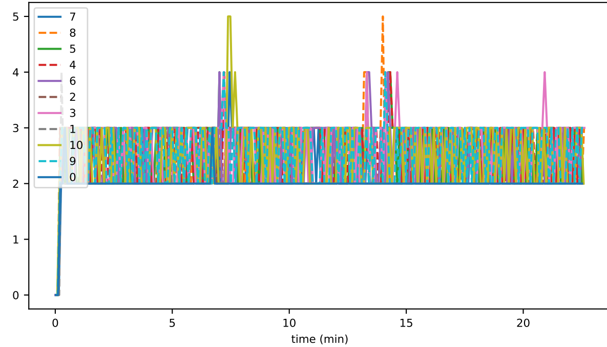
vmap_queries_readEntities_accounts
