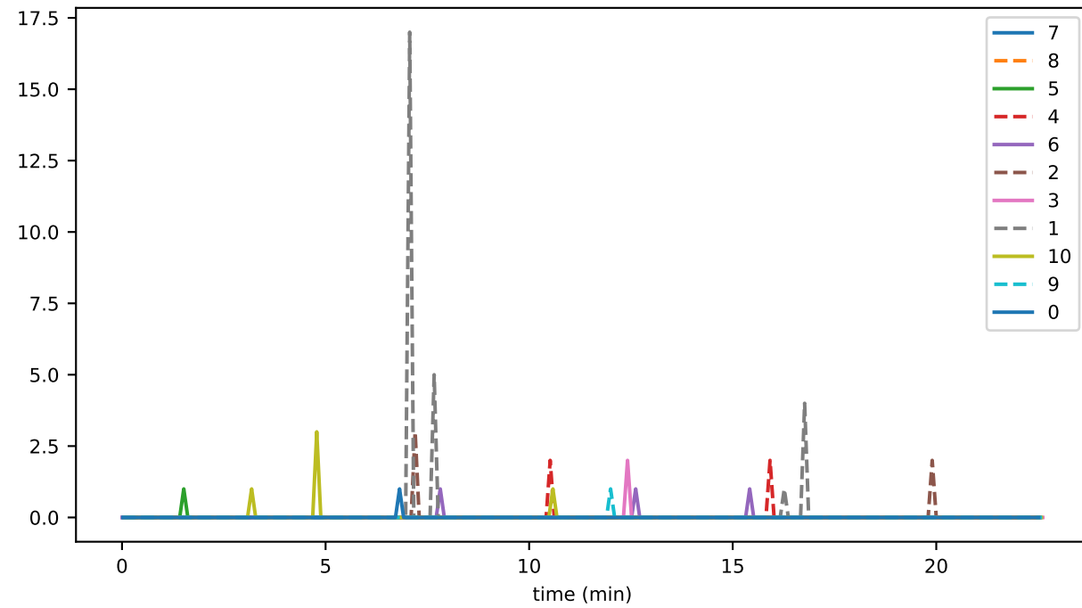
consensusTimeDeviation
