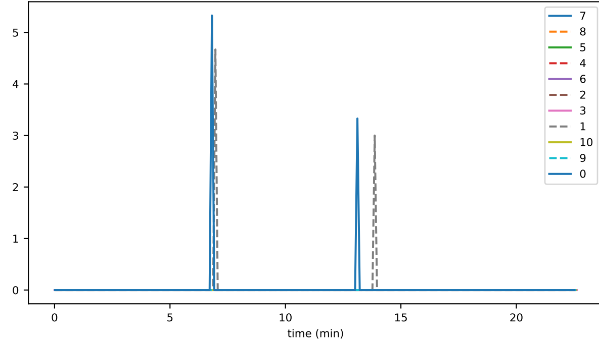
doNotSyncHalted
