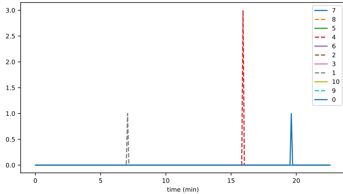
parentBirthRoundMismatch
