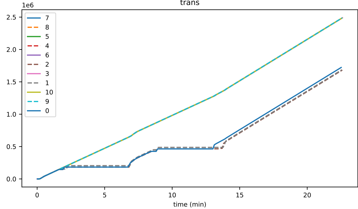
trans_per_event_sys
