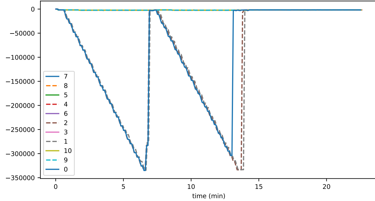
consensusTimeDeviation
