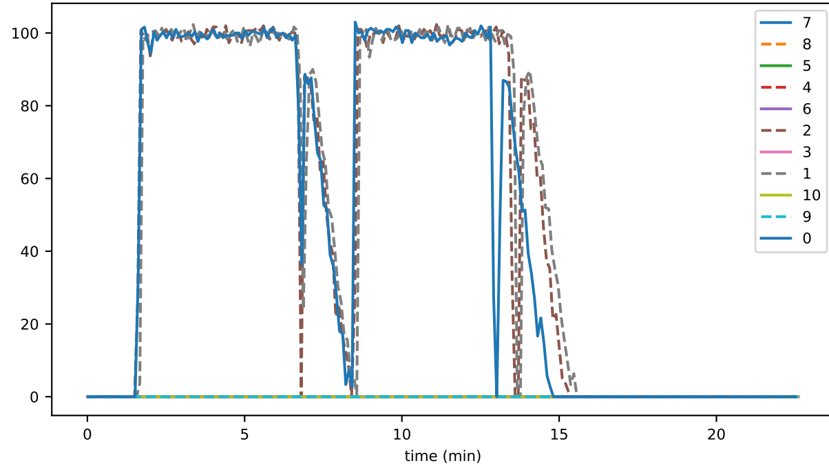
ds_compactions_level_0_hashesSavedSpaceMb_accounts
