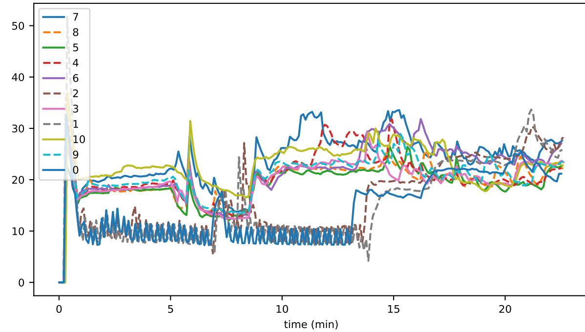
htFCQRecords
