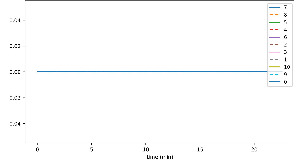
totalNeverSignedDiskStates
