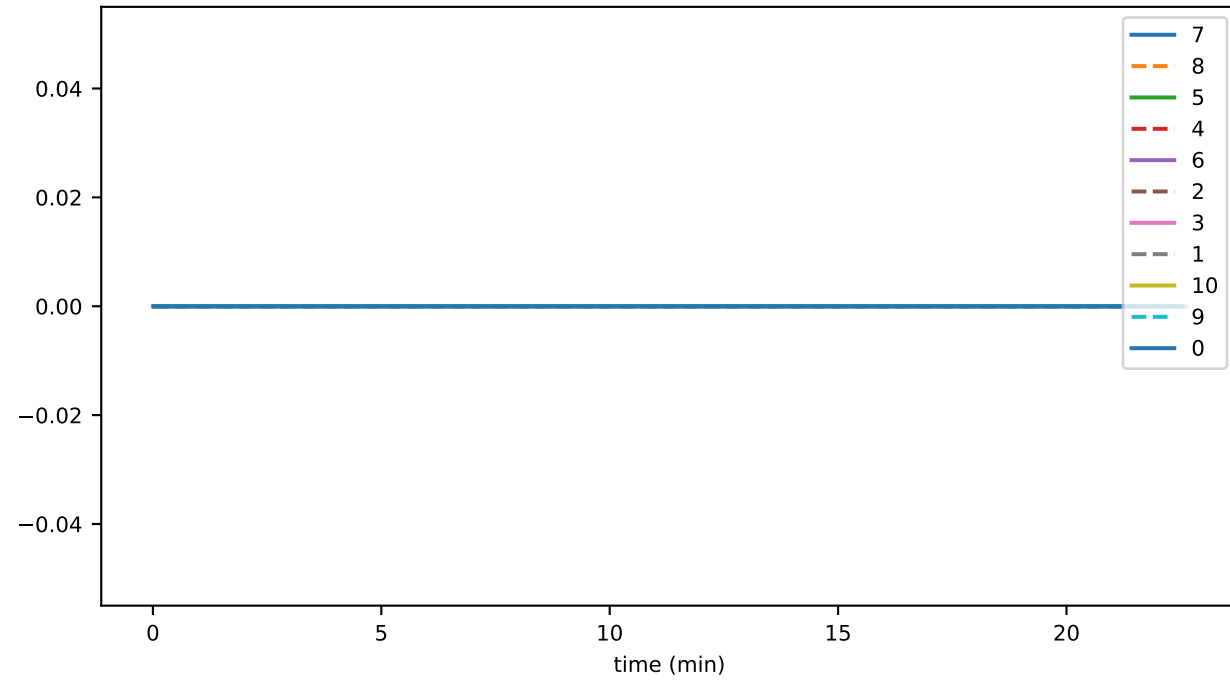
ds_files_level_4_leavesFileSizeByLevelMb_accounts
