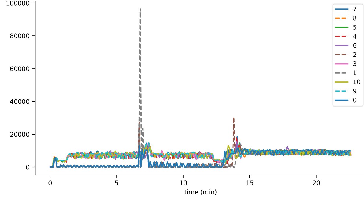
vmap_queries_readEntities_accounts
