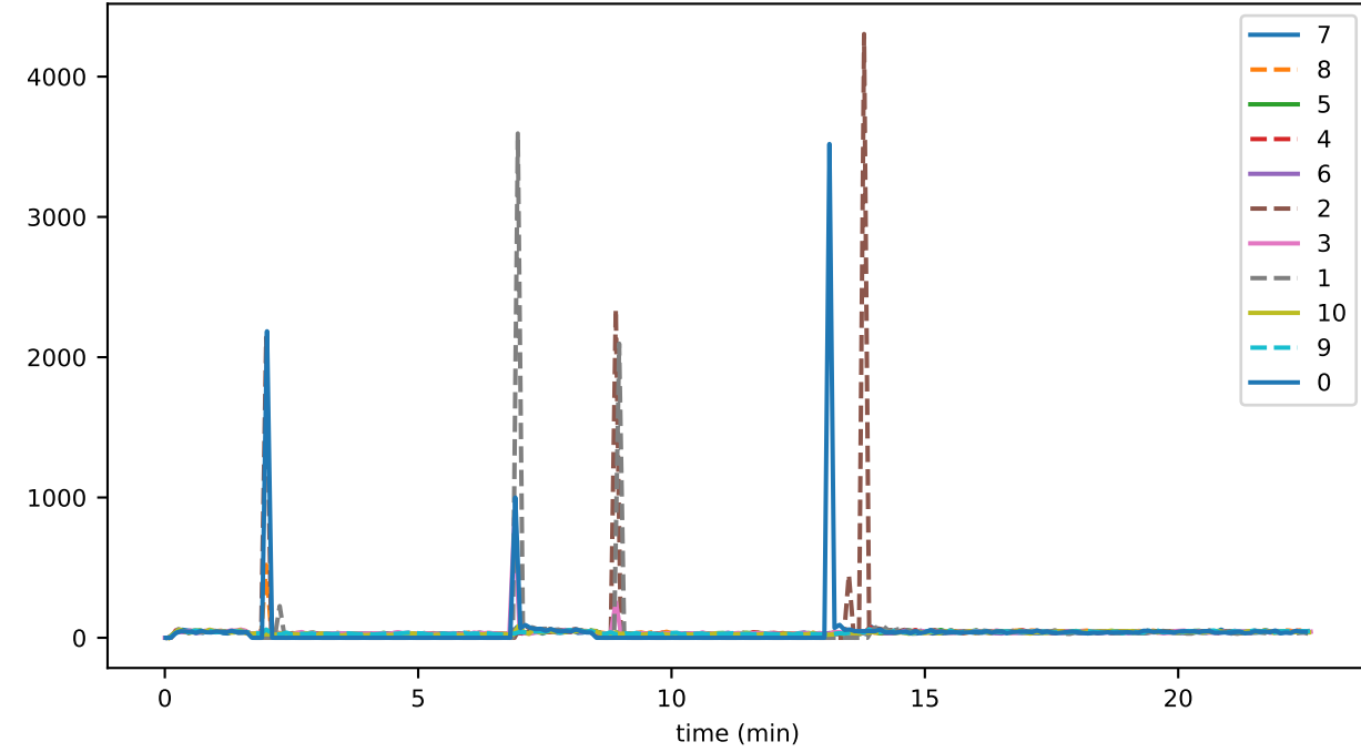
ev_per_syncRMAX
