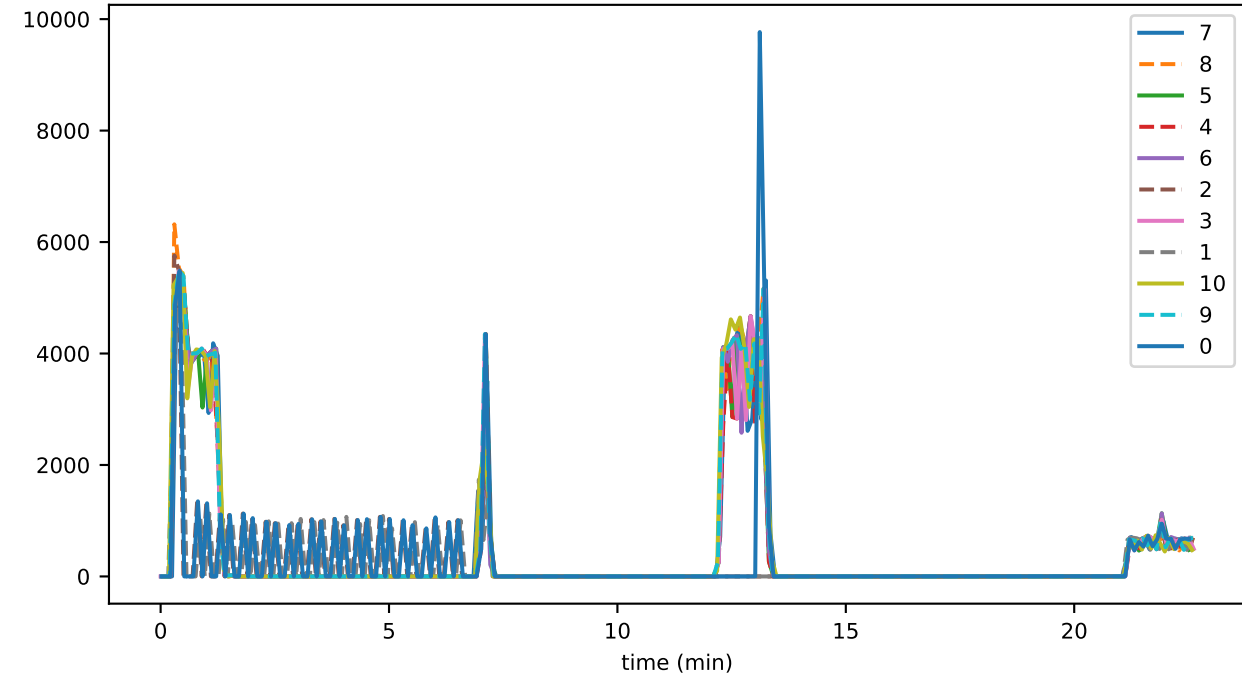
vmap_queries_removedEntities_accounts
