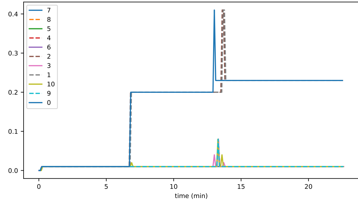
disconnects_per_sec_01
