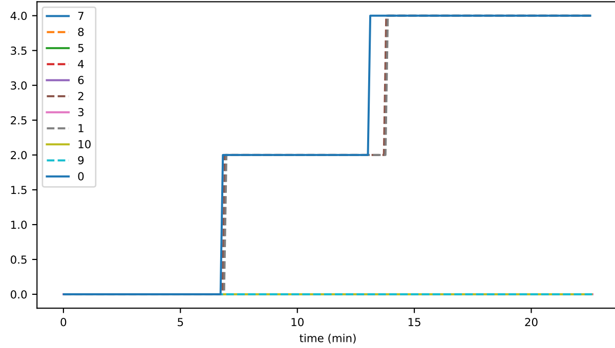
ds_files_hashesStoreFileCount_accounts
