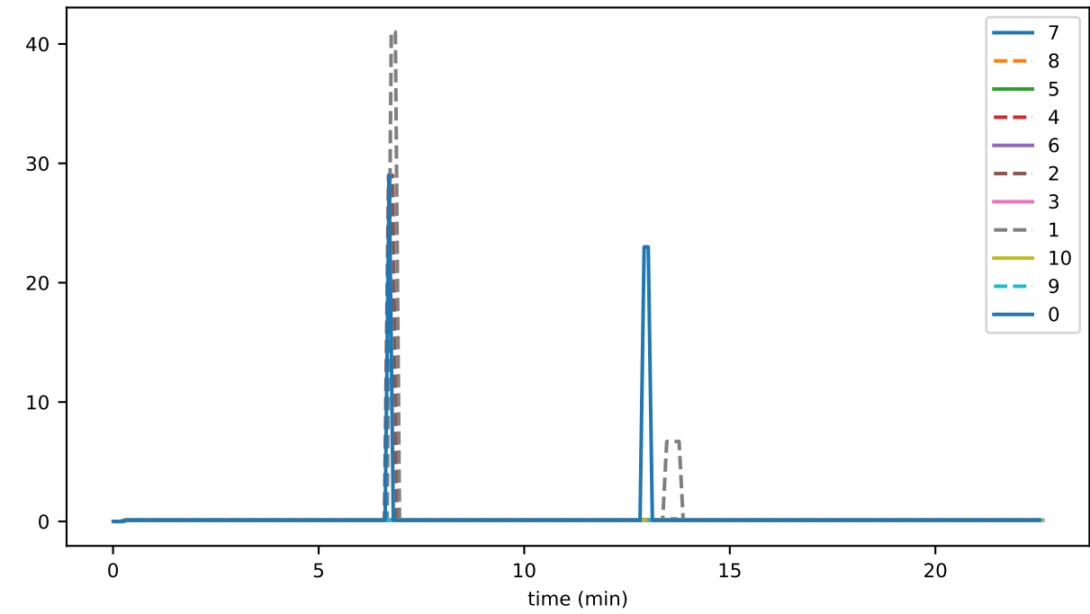
trans_per_event_sys
