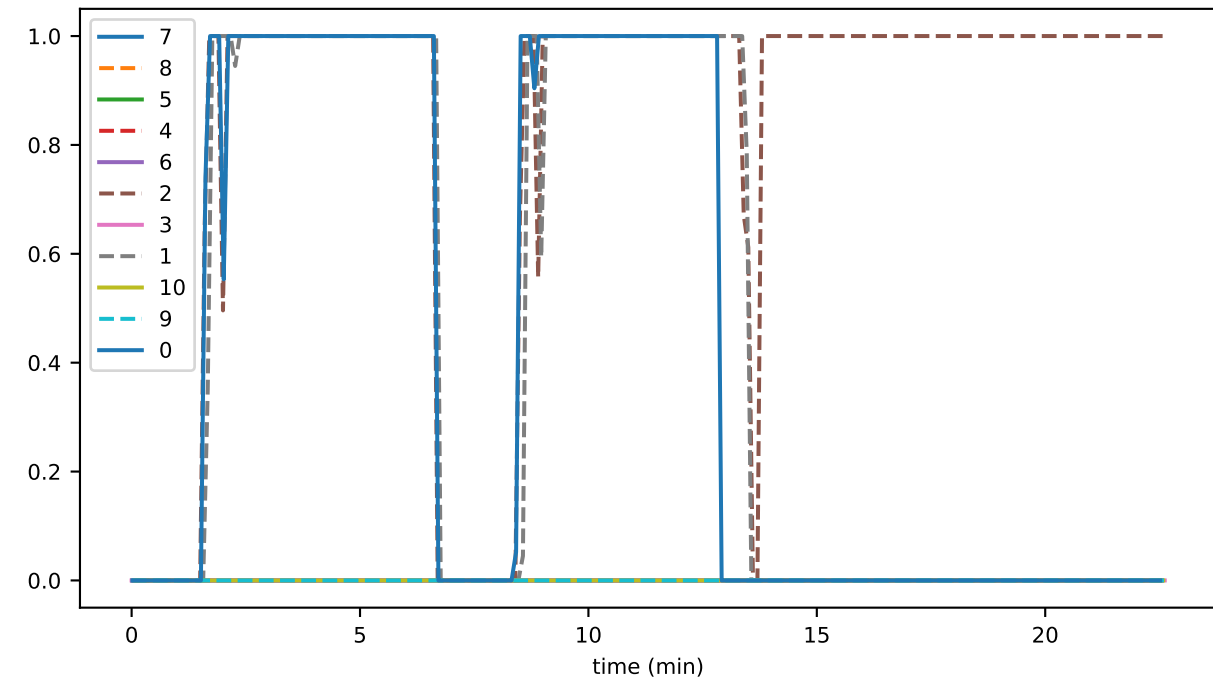
eventCreation_fraction_PLATFORM_STATUS
