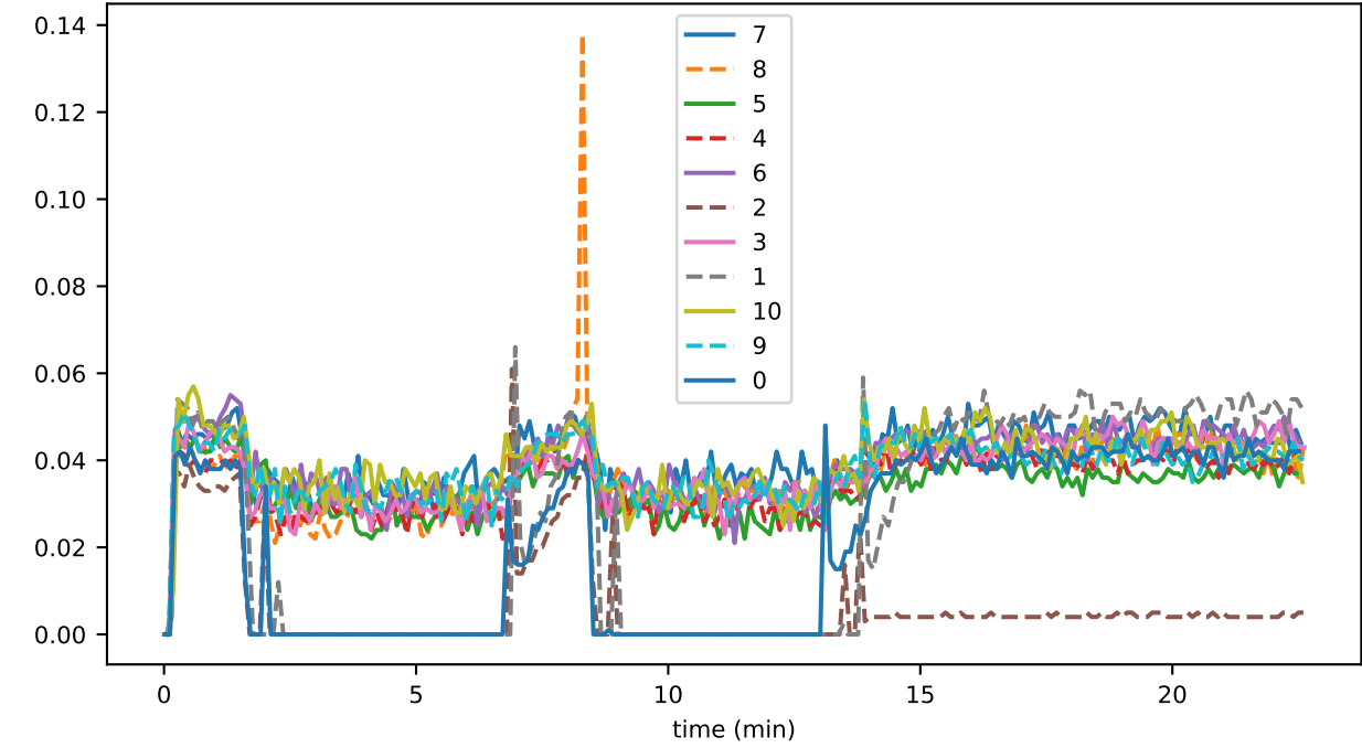
InlinePcesWriter_busy_fraction
