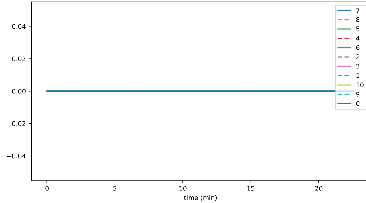
disconnects_per_sec_09
