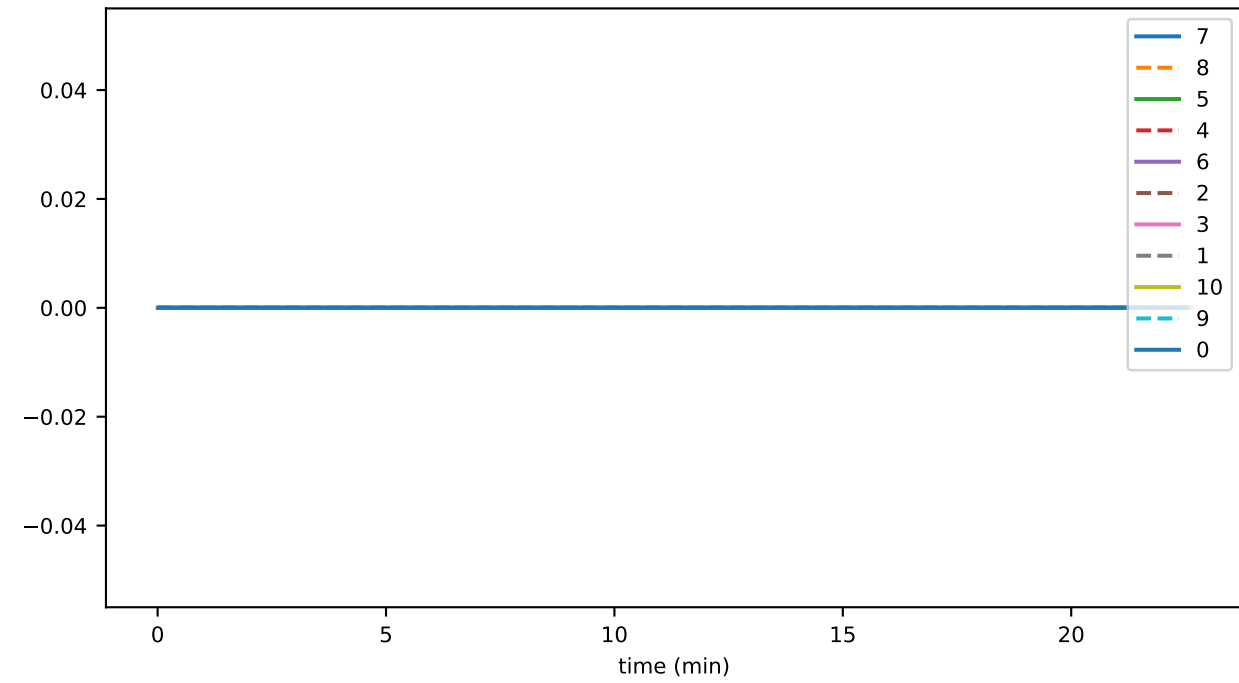
branchingWeightFraction
