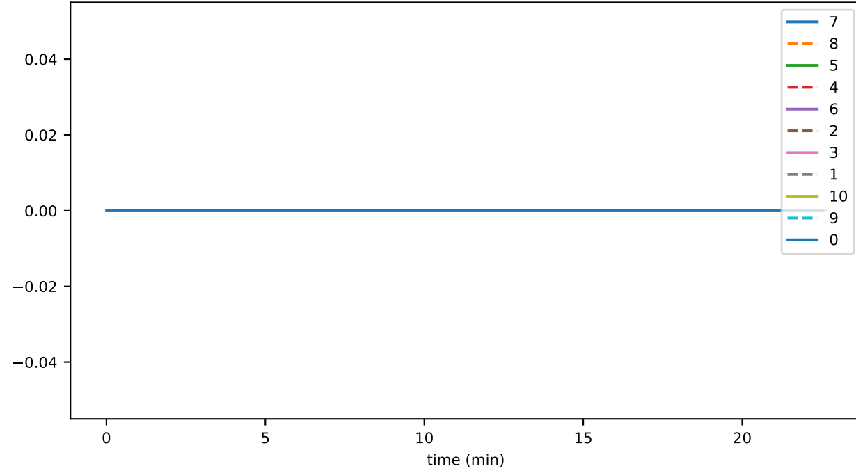
queryLeafTimeCostMicroSec
