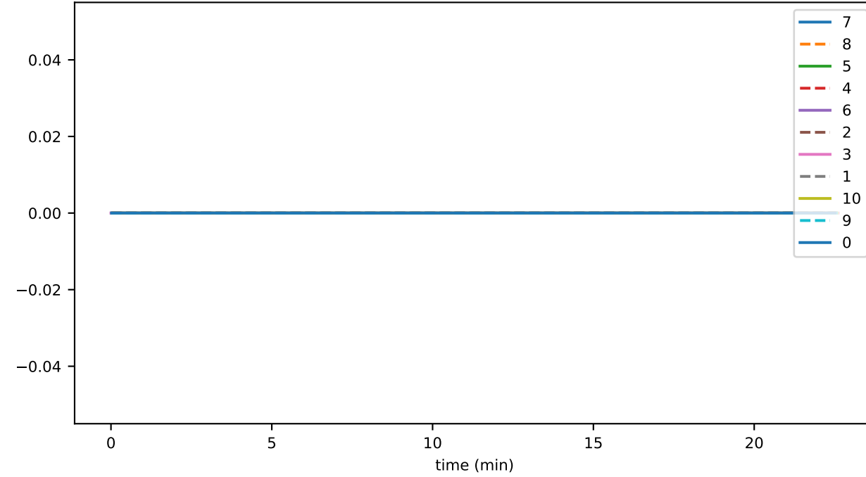
ds_files_level_1_hashesFileSizeByLevelMb_accounts
