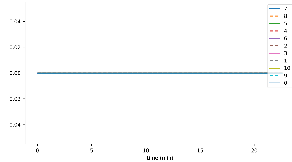
ds_compactions_level_1_leafKeysTimeMs_accounts
