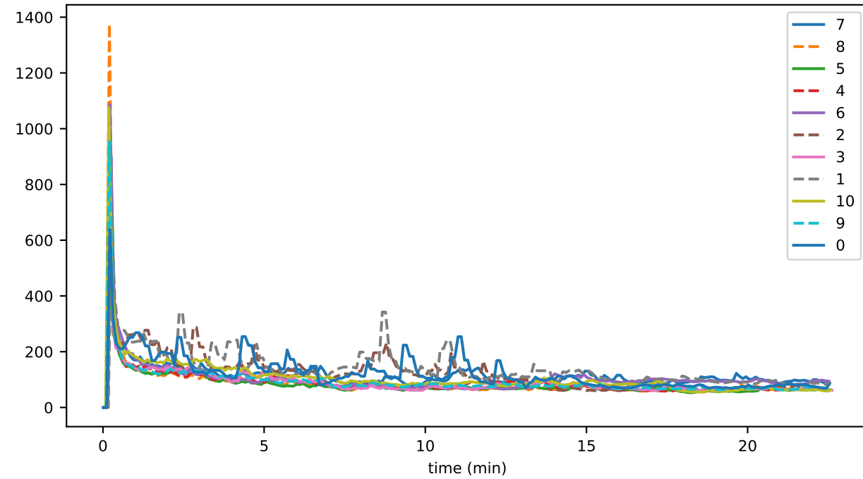
vmap_lifecycle_flushBackpressureMs_accounts
