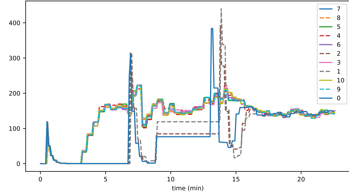
preconsensusEventAverageUnutilizedFileSpan
