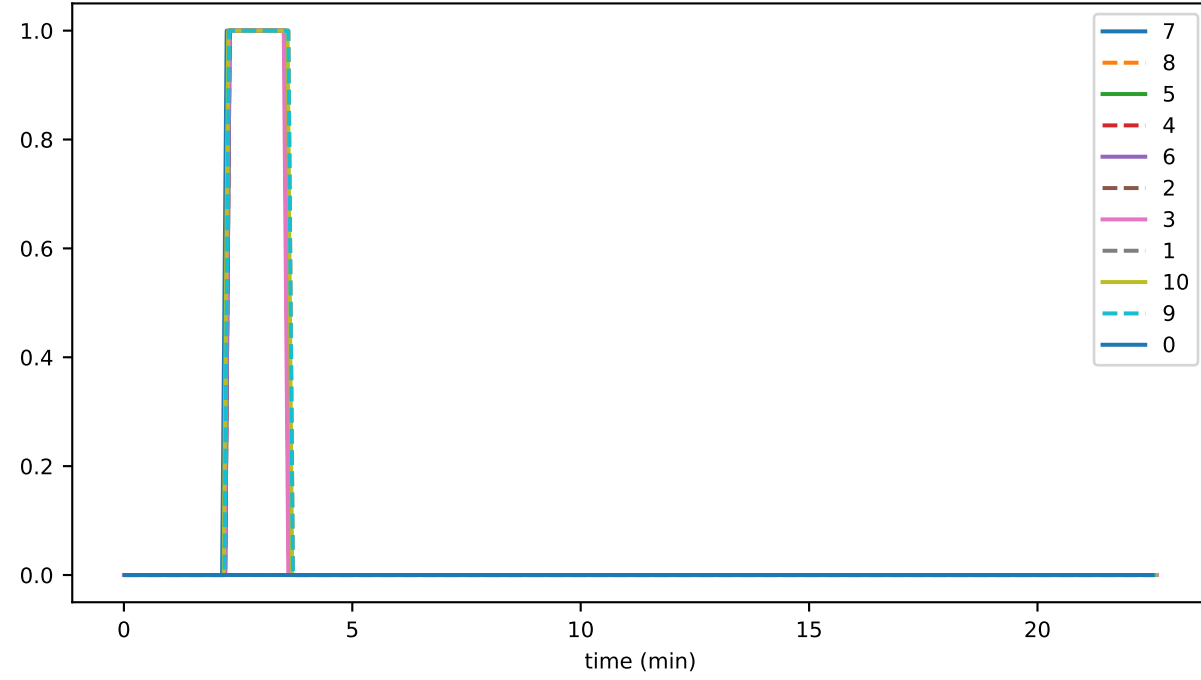
multiTips_per_sync
