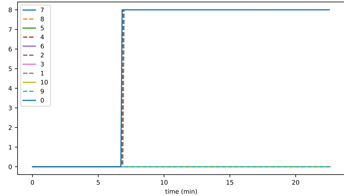
ds_reads_hashes_accounts
