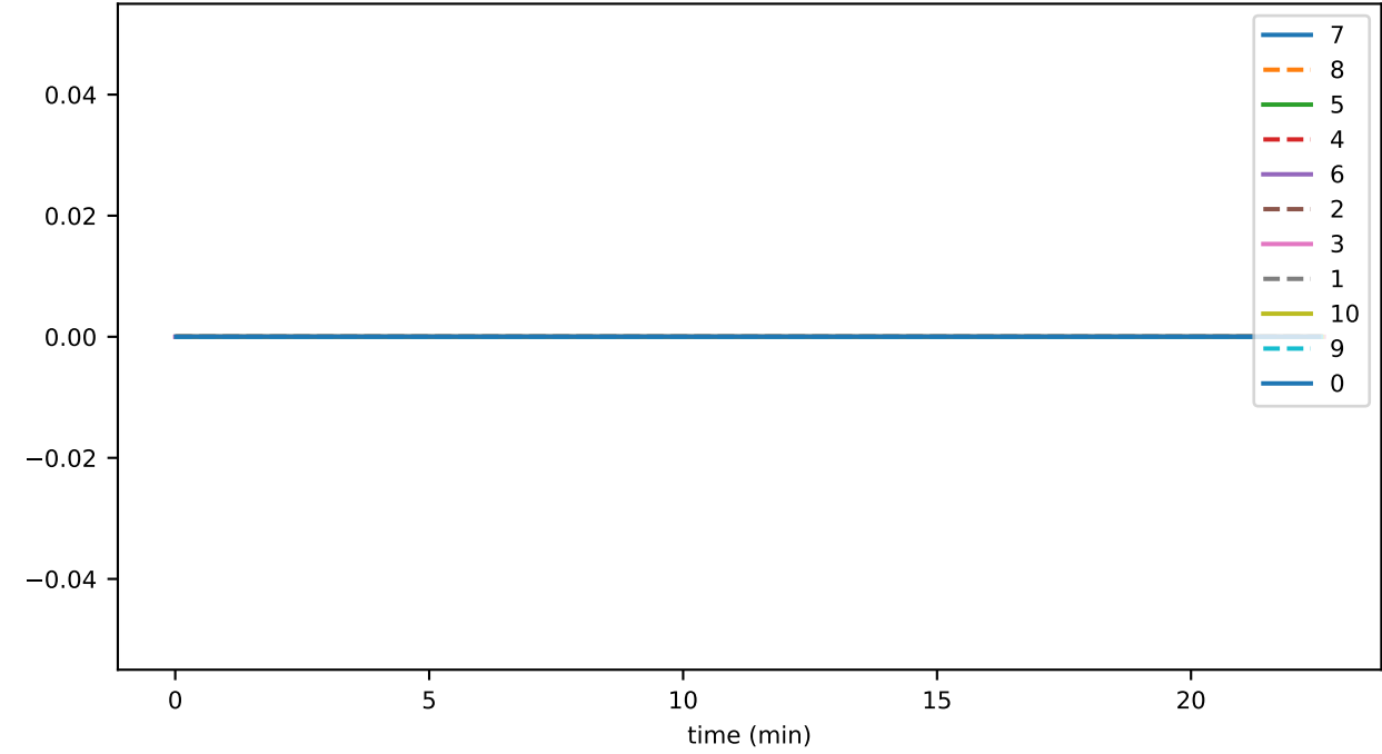
countInMemoryBlockingSwirdState
