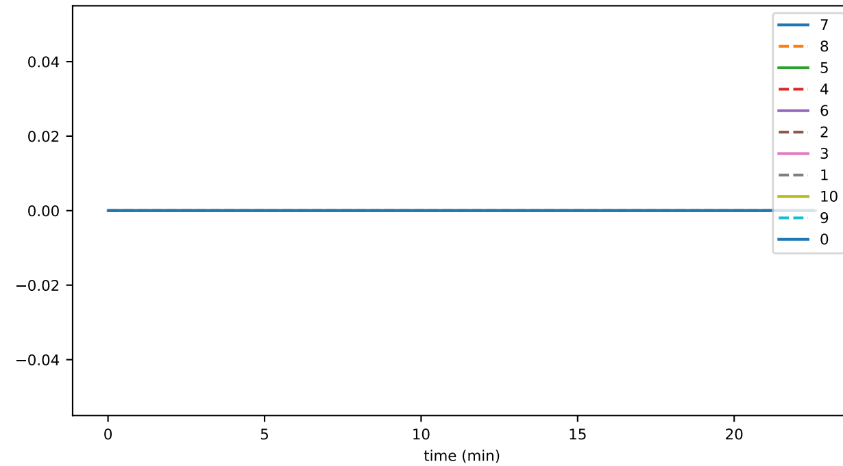
ds_compactions_level_5_leafKeysTimeMs_accounts
