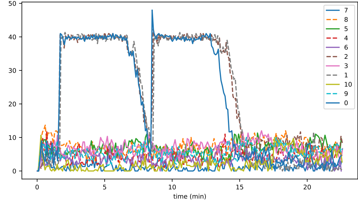
InlinePcesWriter_busy_fraction
