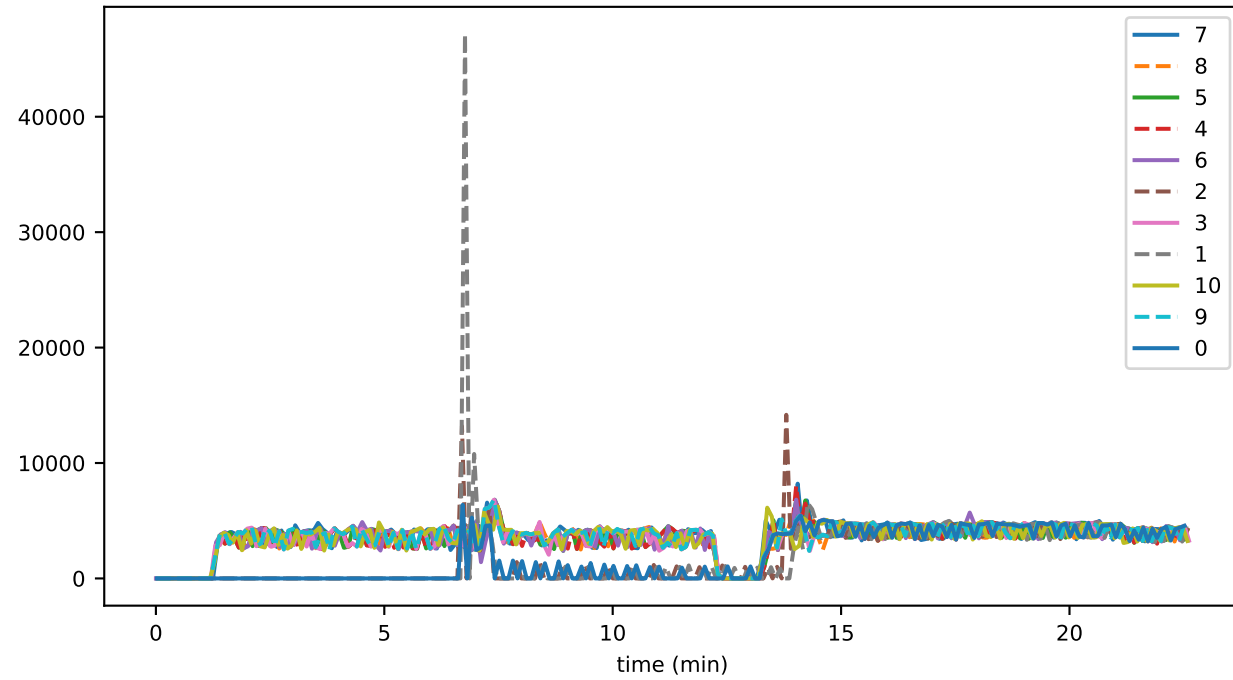
vmContractCreate
