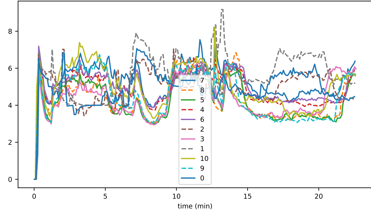
sigStateHash
