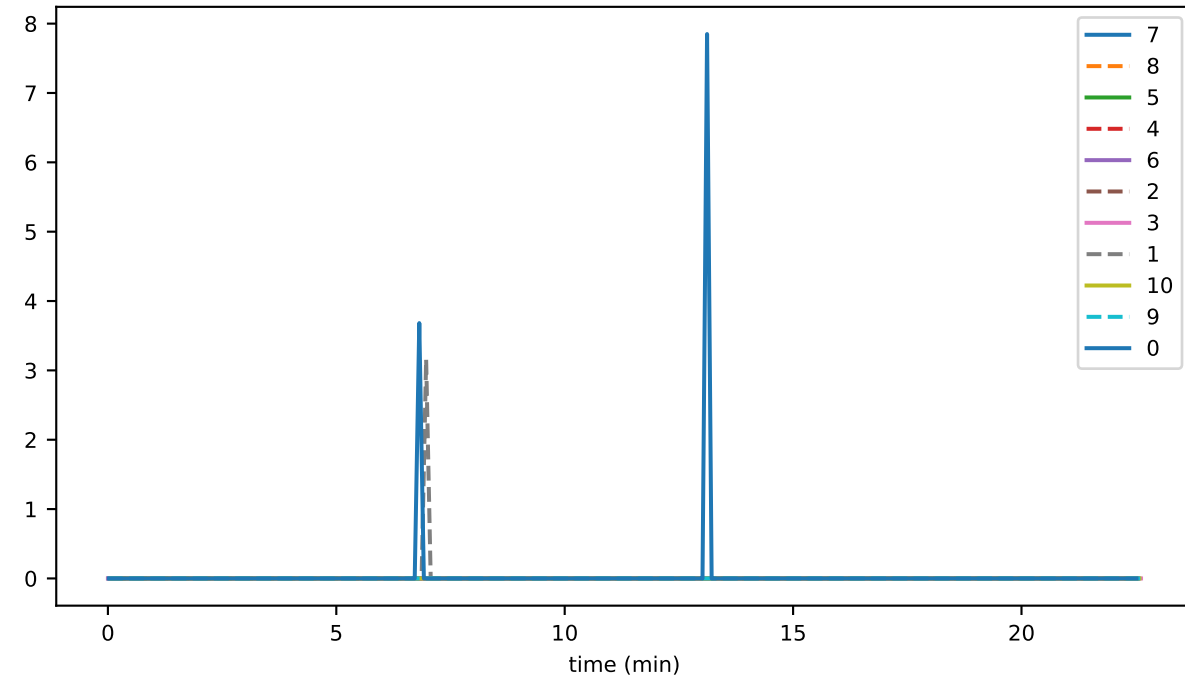
ds_offheap_dataSourceMb_accounts
