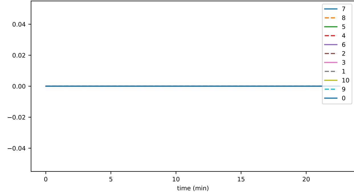
ds_reads_hashes_accounts
