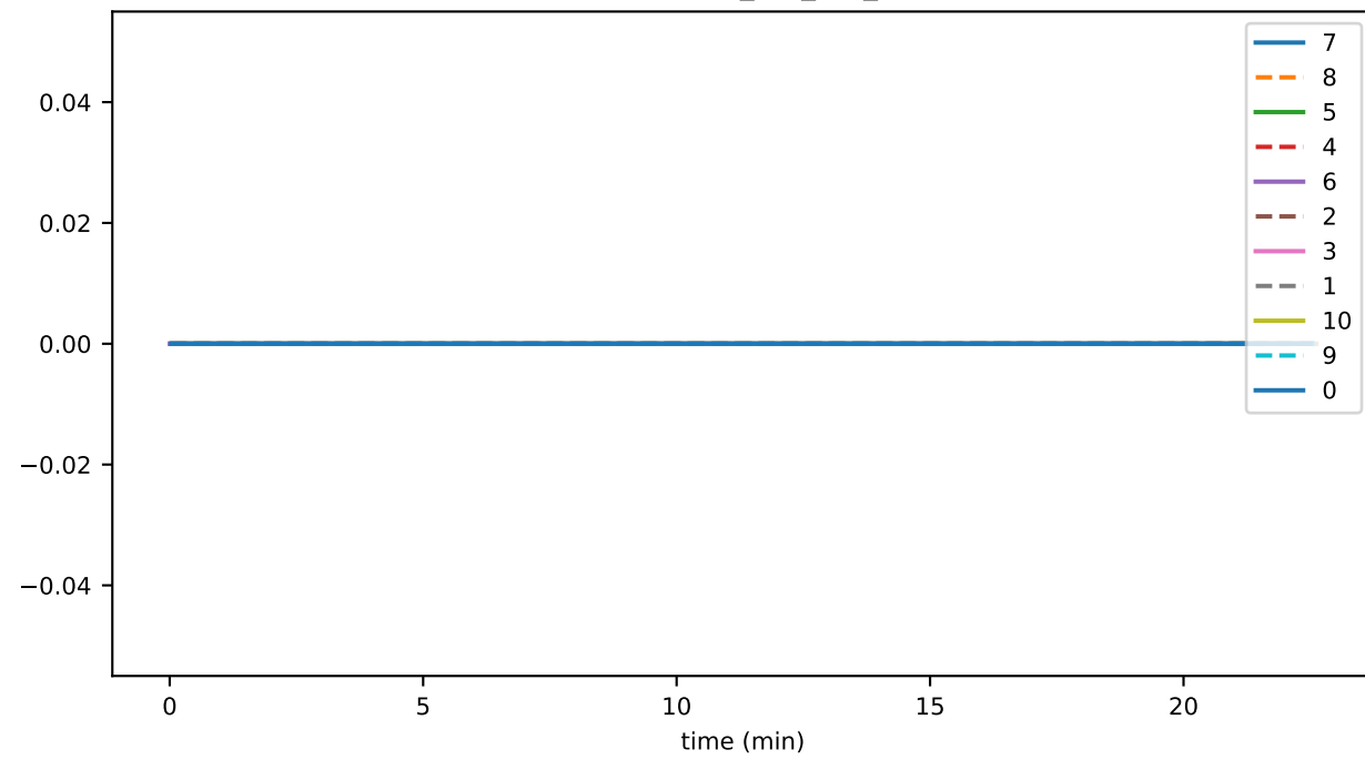
disconnects_per_sec_04
