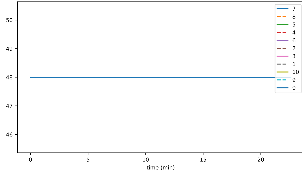
queryLeafTimeCostMicroSec
