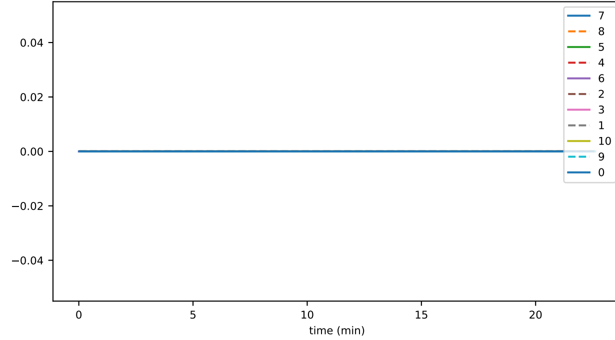
nftBurnTokenMicroSec
