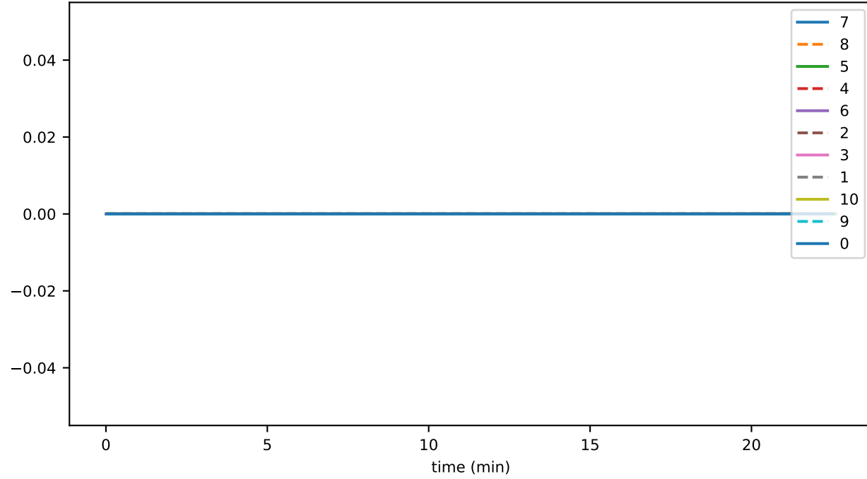
roundsSinceLastConsensusEvent_10
