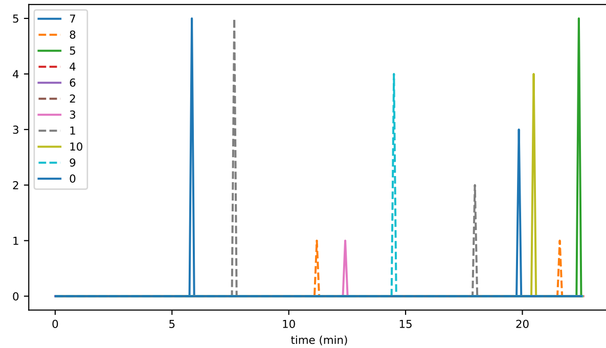
branchingNodeCount
