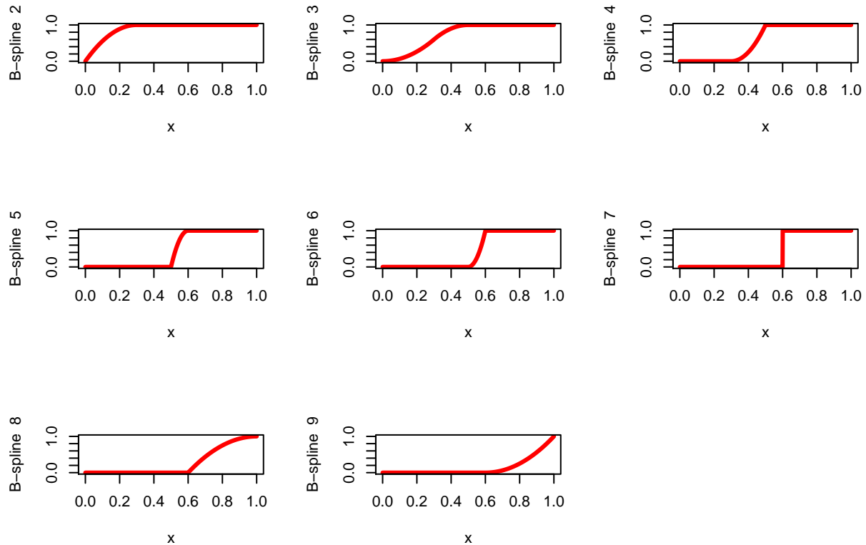
Figure 15: Monotone Piecewise Quadratic Splines with Multiple Knots
