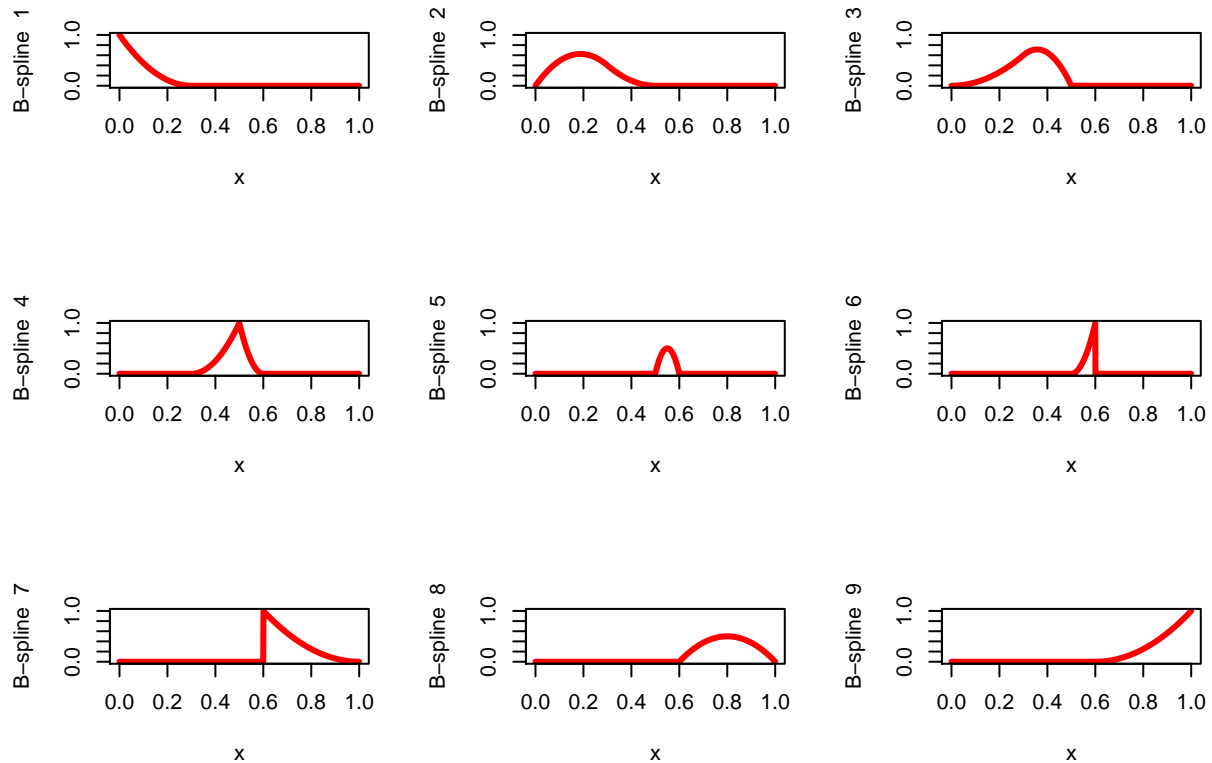
Figure 10: Piecewise Quadratic Splines with Multiple Knots
