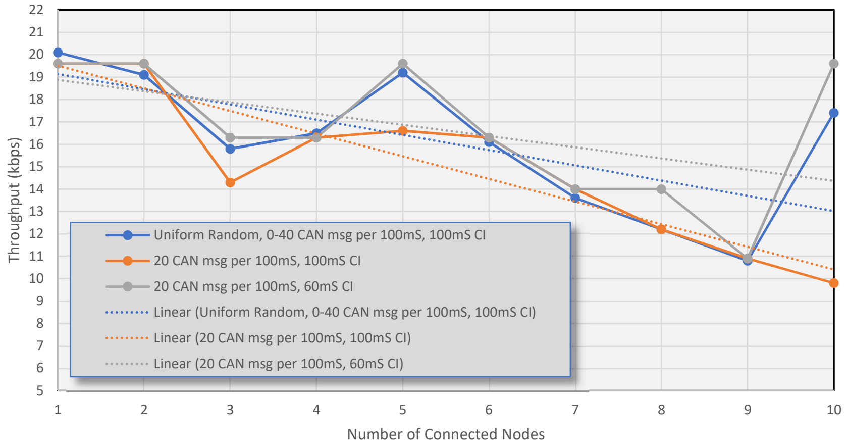
BLE Throughput vs Connected Nodes (Nominally 20kbps b > n , 4.7kbps n > b )
